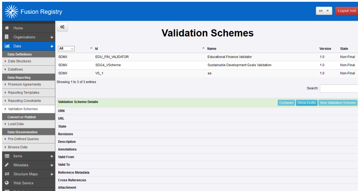
Figure 1 – Showing example Validation Schemes in the Fusion Registry
