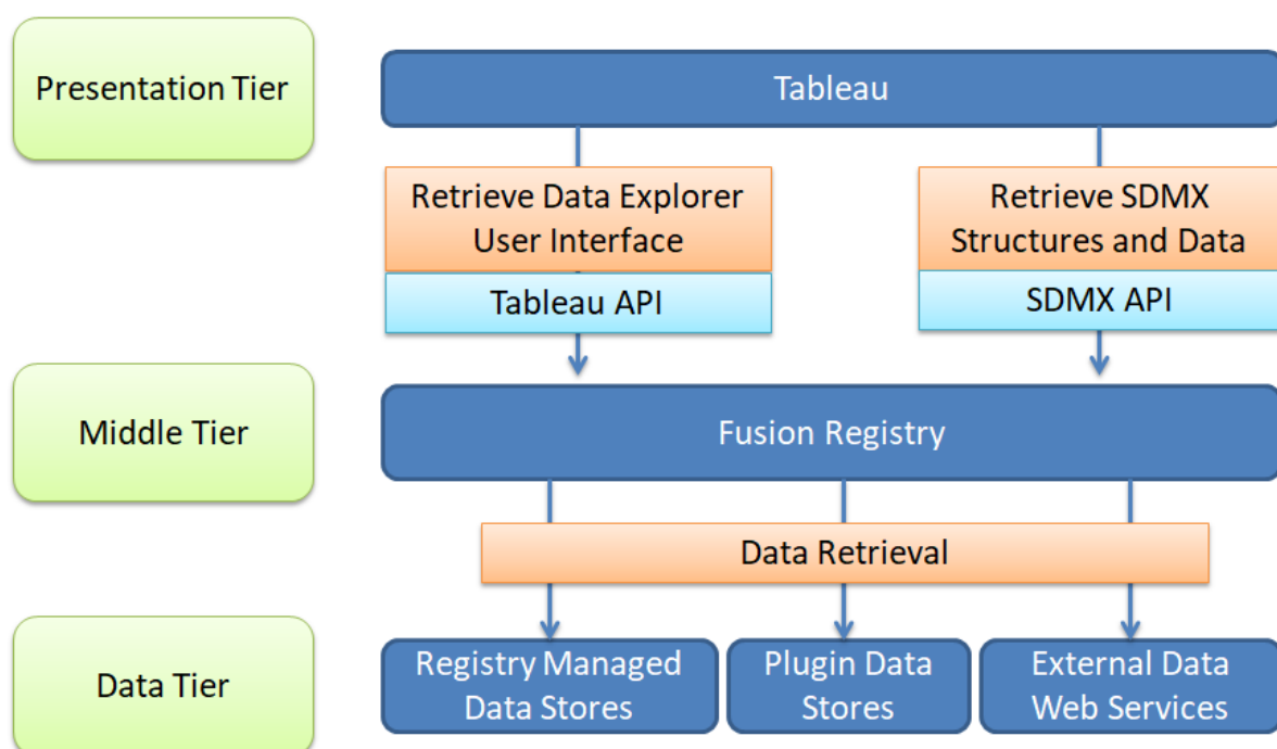
Figure 1 showing a high level architecture of Tableau connectivity to the Fusion Registry
